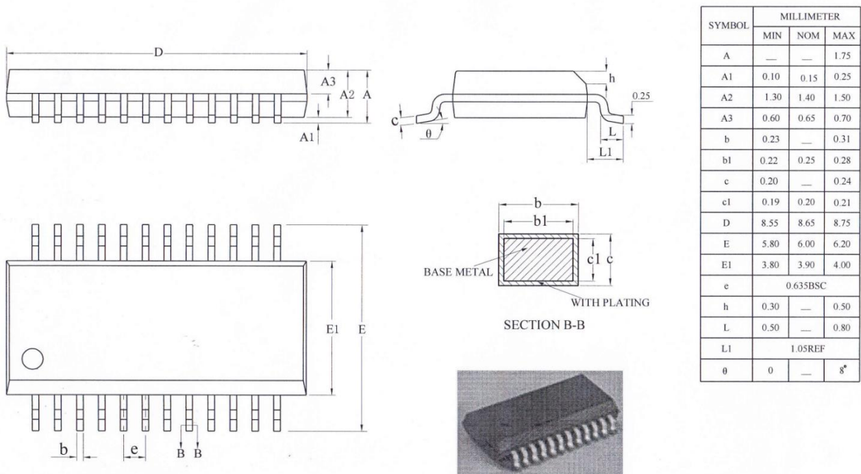
Figure 3-1 HA3616D SSOP24 Package
