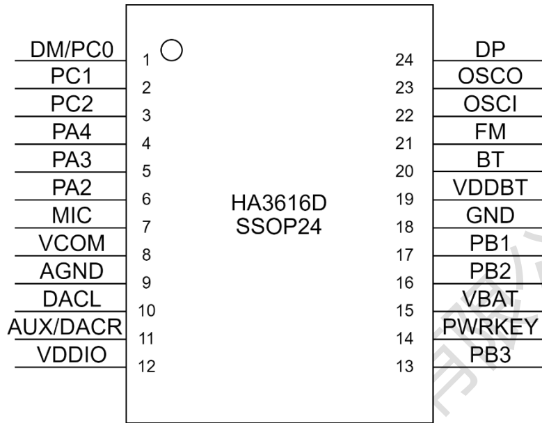
Figure 2-1 HA3616D SSOP24 Pin assignment
